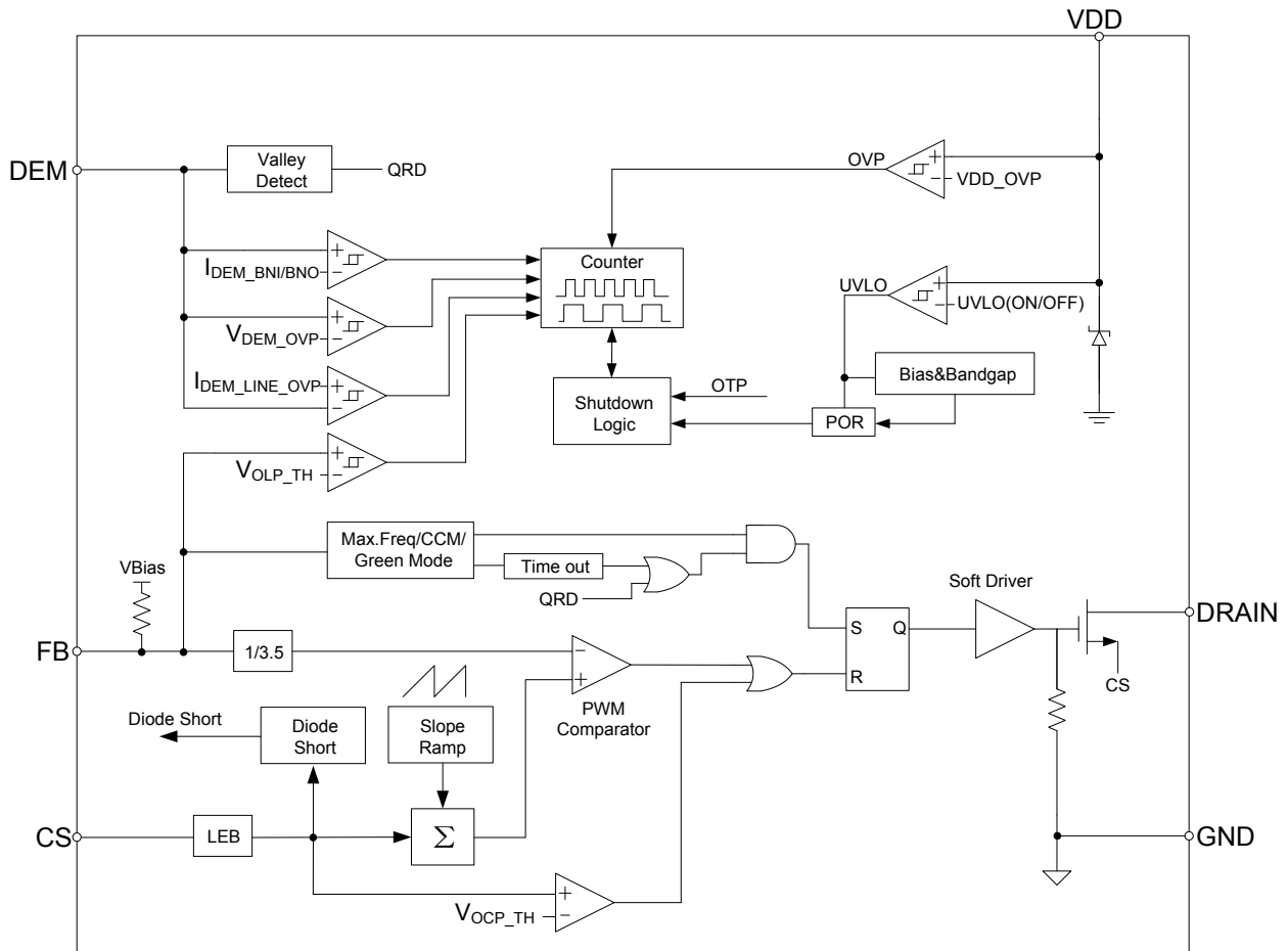
Figure 2. Block diagram of SP6668P
