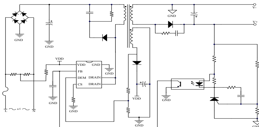
Figure 1.Simplified Application of SP6668P
